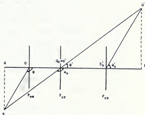
Fig. 1. Kantor's experiment.
