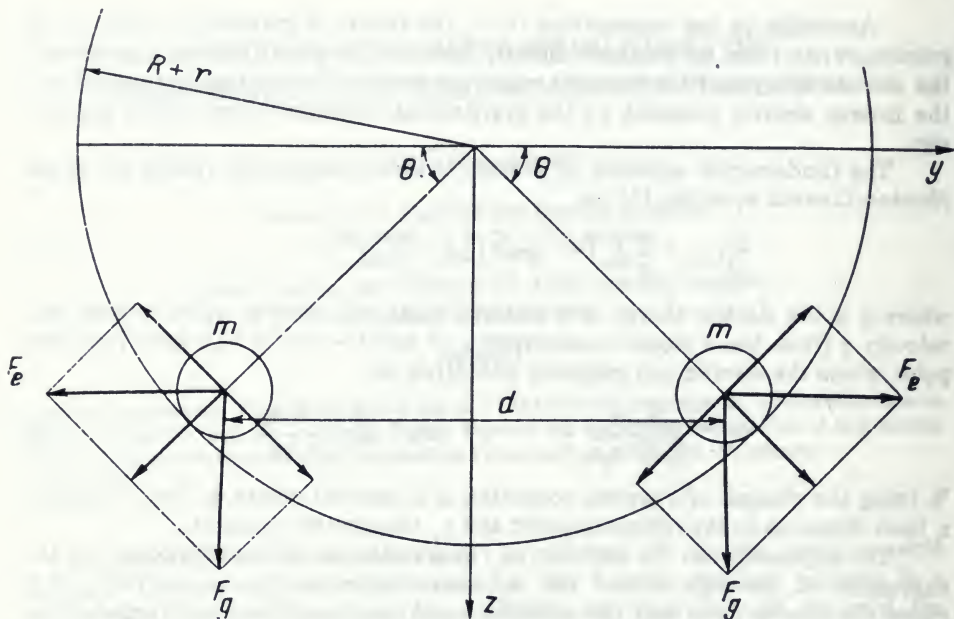
Figure 1. The "cauldron" experiment.
