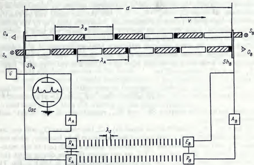
Figure 1. The ultrasonic "coupled-shutters" experiment.
