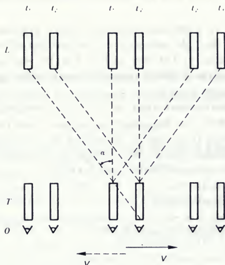
Fig. 1. Wilczyński's experiment analyzed in absolute space.
