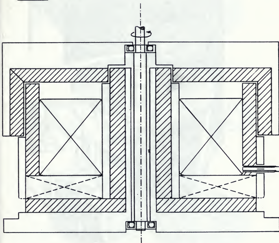
Fig. 17. - Diagram of the second VENETIC COLIU machine. The diameter of the rotor is 18 cm.
