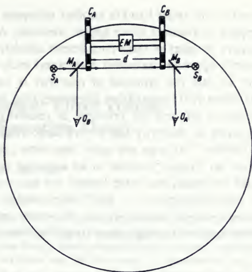
Fig. 8. Coupled shutters mounted on a rotating disk for d much less than 2\pi R .
