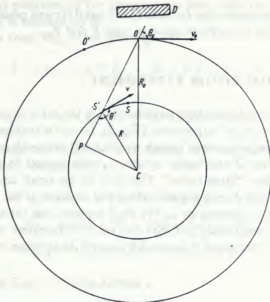
Fig. 4. The rotor experiment.
