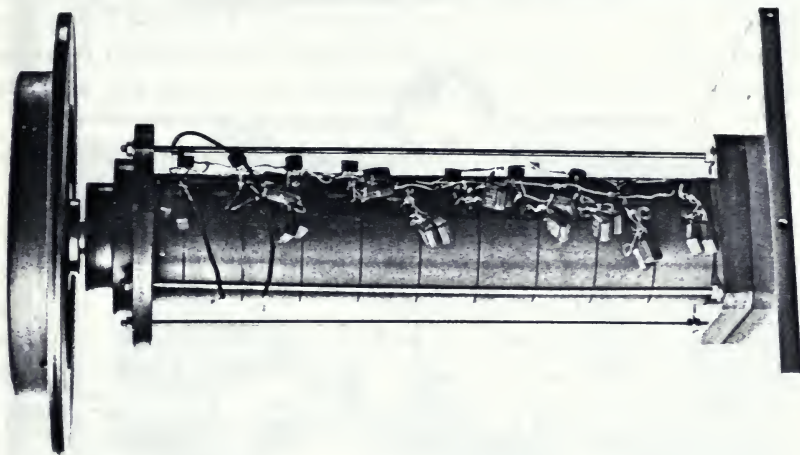
Fig. 5. - The same machine as in fig. 4, where the driving motor sets in motion a fly-wheel, so that all losses are reduced to a minimum.
