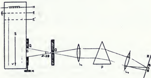
Fig. 1. Scheme of the experiment for the establishment of the zero transverse light Doppler effect.
