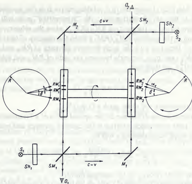
Fig. 1. The interferometric "coupled-mirrors" experiment.
