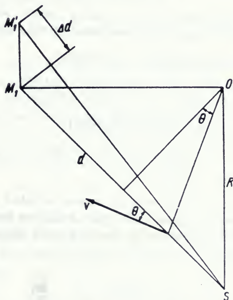
Fig. 3. Detail of the rotating disk experiment.
