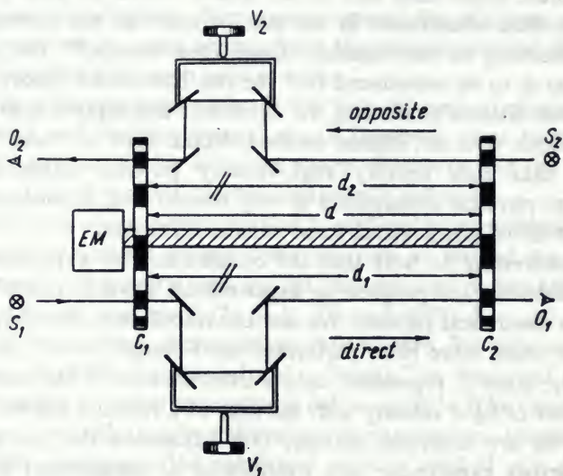
Fig. 5. Rigidly connected coupled shutters.
