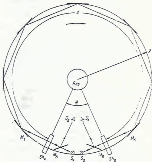
Fig. 1. The "coupled-shutters on a rotating disk" experiment.
