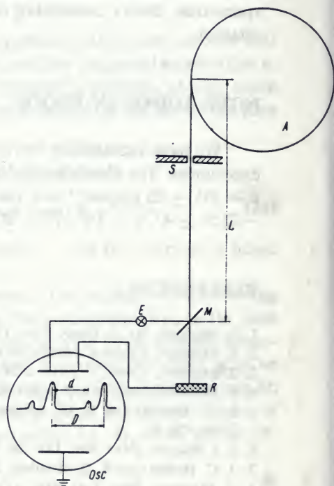
Fig. 1. The "synchrotron" experiment.
