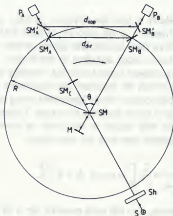
Figure 1. The interrupted 'rotating disc' experiment.
