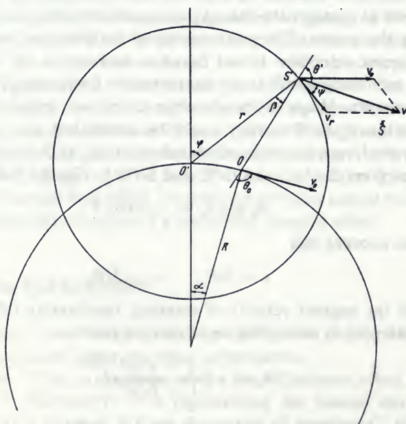
Fig. 5. The rotor-rotor experiment.
