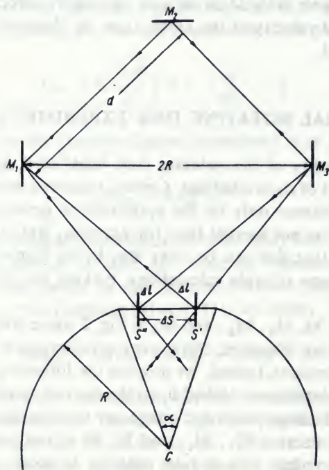
Fig. 4. The inertial rotating disk experiment.
