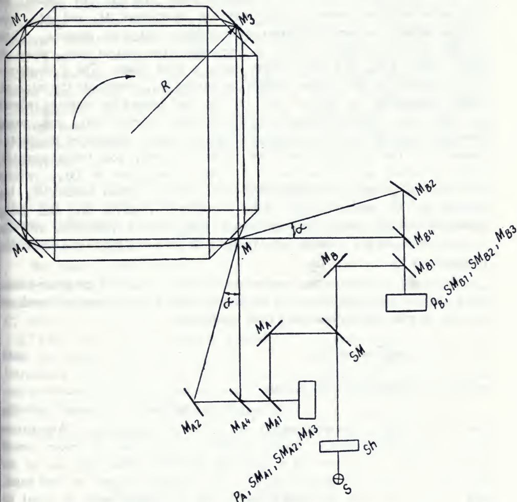
Figure 2. Actual scheme of the "moving platform" experiment (the non-inertial "moving platform" experiment).
