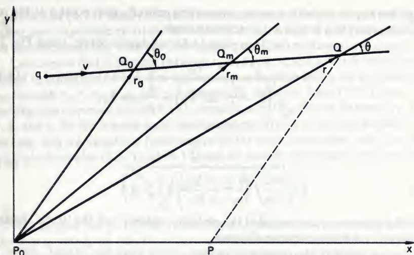
Figure 2.—A 'photon-runner' going 'there' or 'back'.
