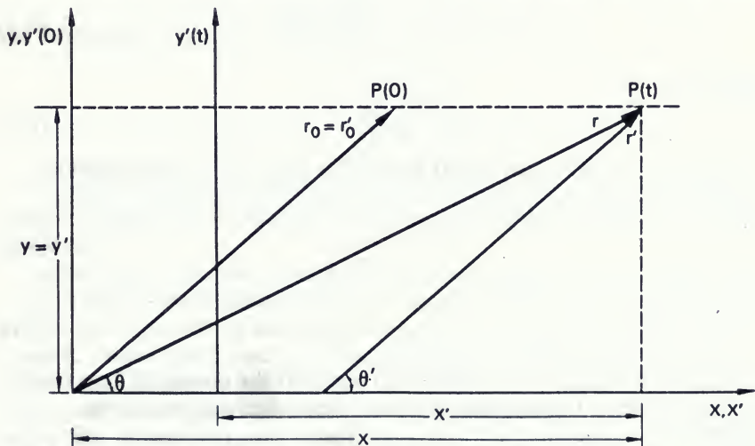
Figure 1.—Two space frames moving with respect to each other, the transformation between being a special one.
