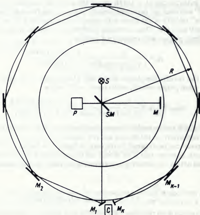
Fig. 2. The setup for the measurement of the second-order effects on the rotating disk.
