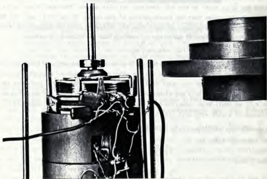
Fig. 14. - One of the Bosch generators (the tenth in VENETIN COLIU - I) with the original Bosch coil on which additional windings were wound.
