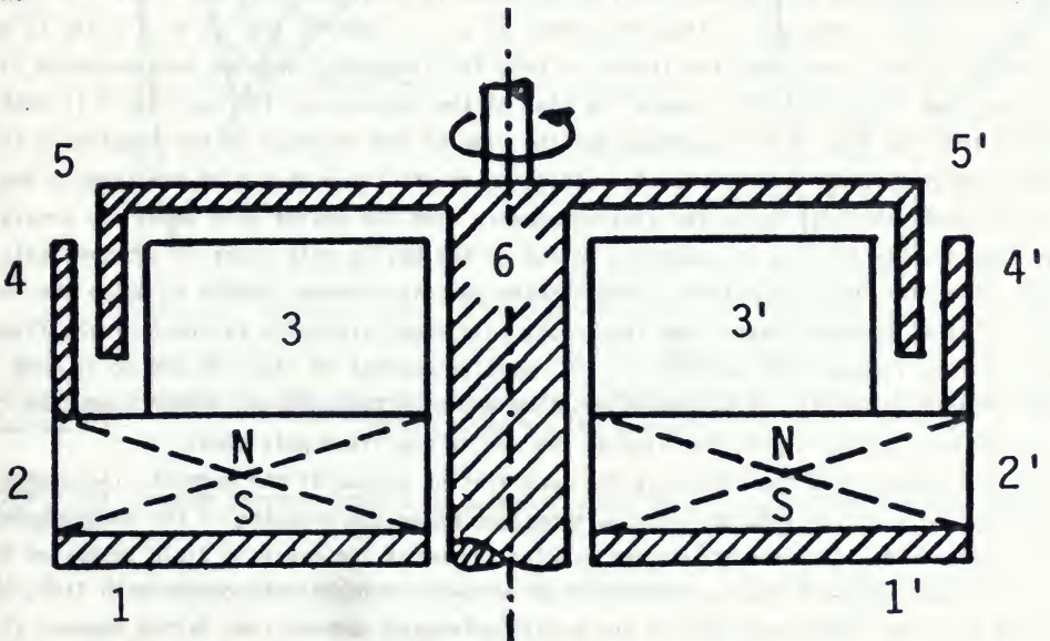
Fig. 2. Diagram of the generator VENETIN COLIU.
