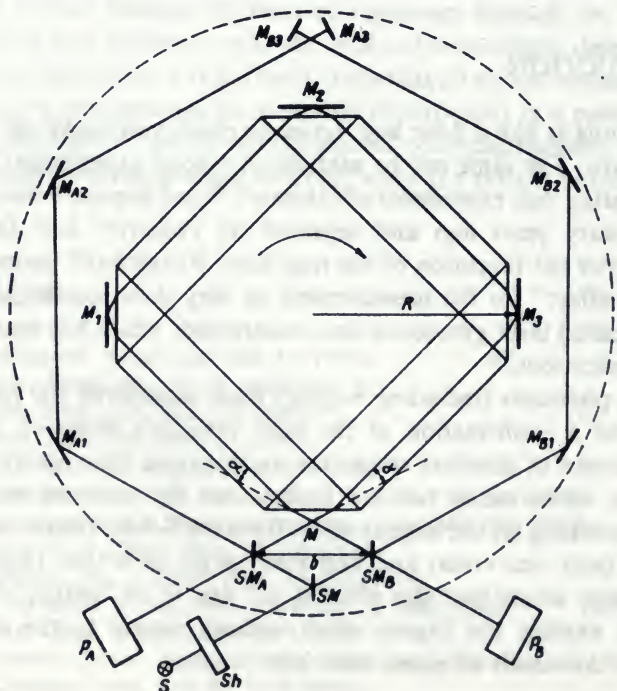
Fig. 1. Scheme of the rotating disk experiment in our version.
