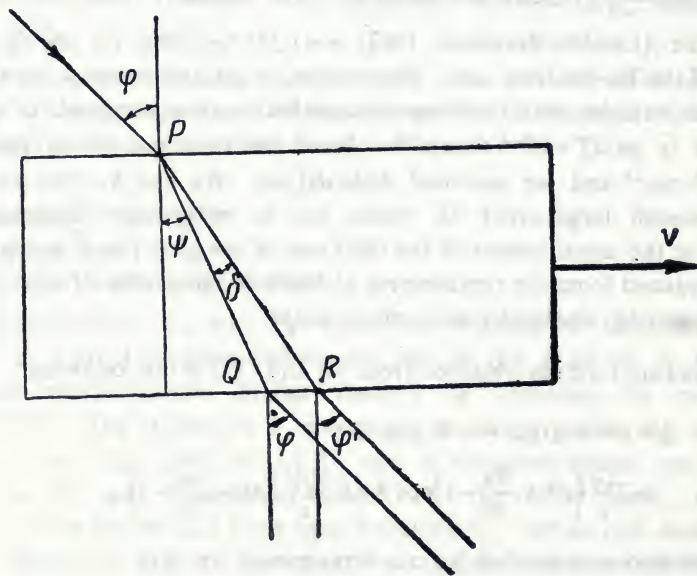
Figure 3. The drag aberration.
