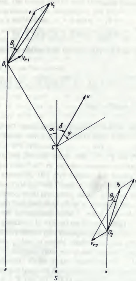
Fig. 1. The quasi-Doppler experiment.
