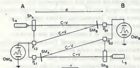
Fig. 1. Set-up of a "synchronous light clocks" experiment.
