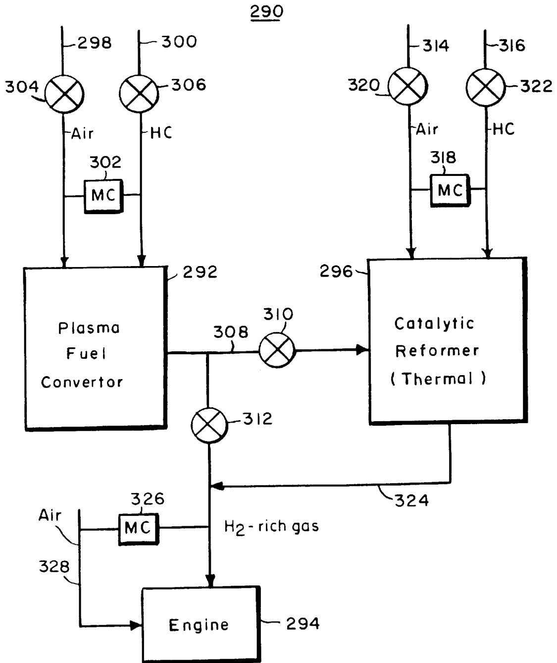
Hybrid Plasma Fuel Converter - Catalytic (Thermal) Partial Oxidation Reformer
