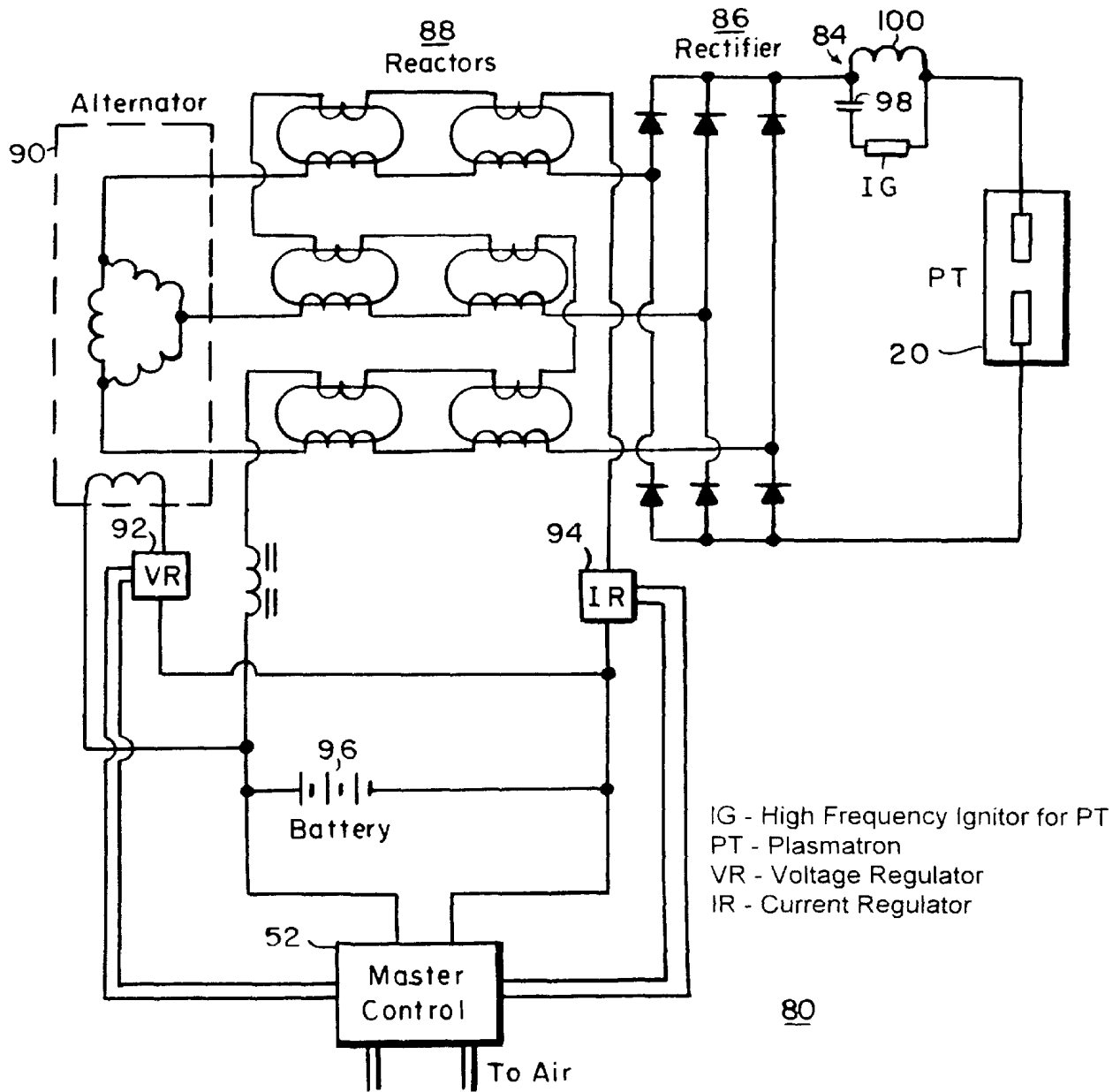
Power Control Circuit for Continuous Arc Plasma Fuel Convertor
