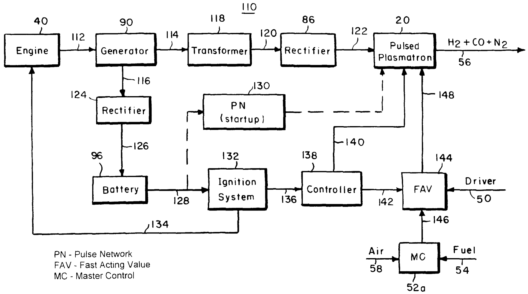
Pulsed Plasmatron - Engine Electrical System
