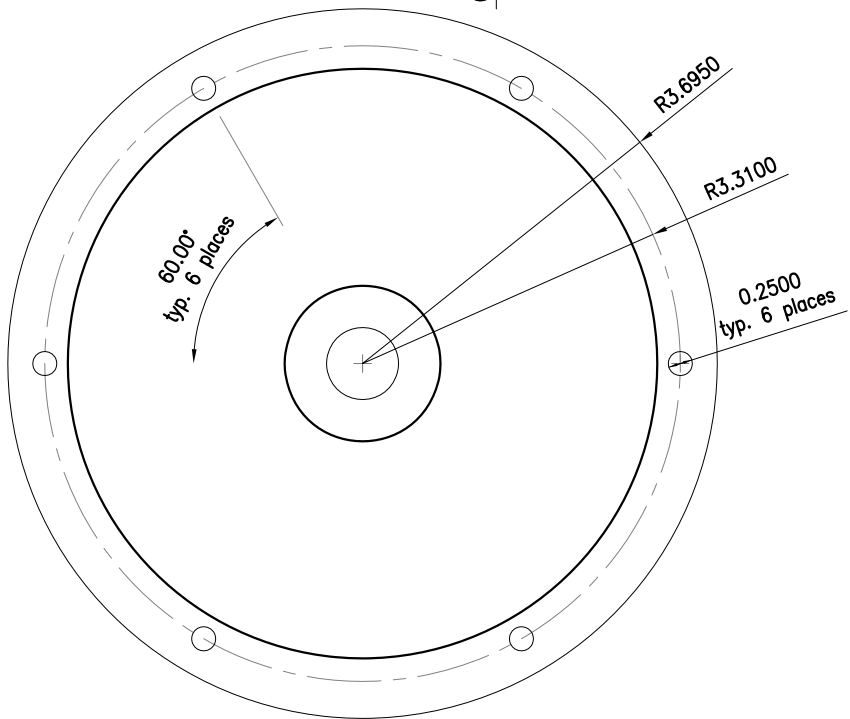
Permag 7" Motor Front Plate
