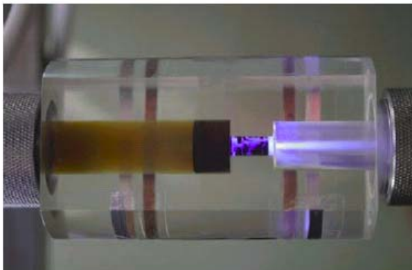
Figure 5. Generation of the directed bright light beam in the turbulent machine oil
