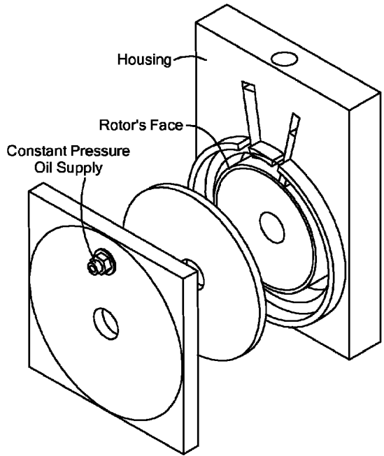
Exploded Front View
