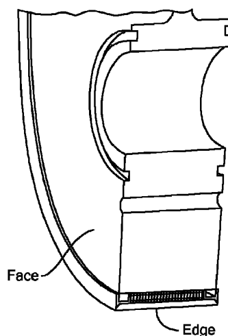
Wedge profile face seal
