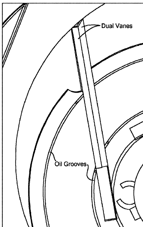
Dual Vanes help to seal against housing. Two vanes are in sliding contact with each other, which could be enhanced by oil film. Oil is delivered through the grooves.
