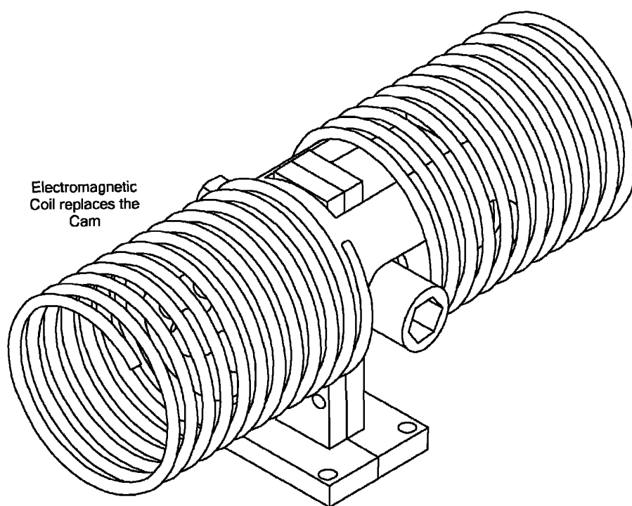
Single Piston with Electromagnetic Coil Embodiments
