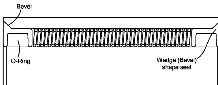
Wedge seal cross section
