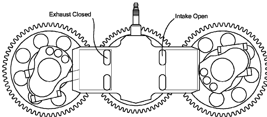
Two Pistons - Opposed Pistons Embodiment. Intake Stroke
