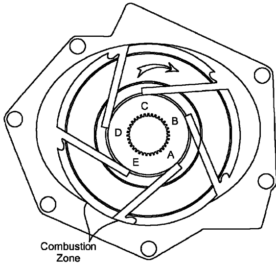
General View FIG. 38A
