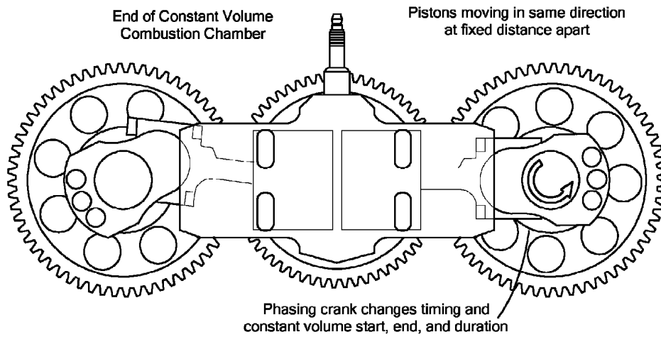
Two Pistons - Opposed Pistons Embodiment. Constant Volume Combustion
