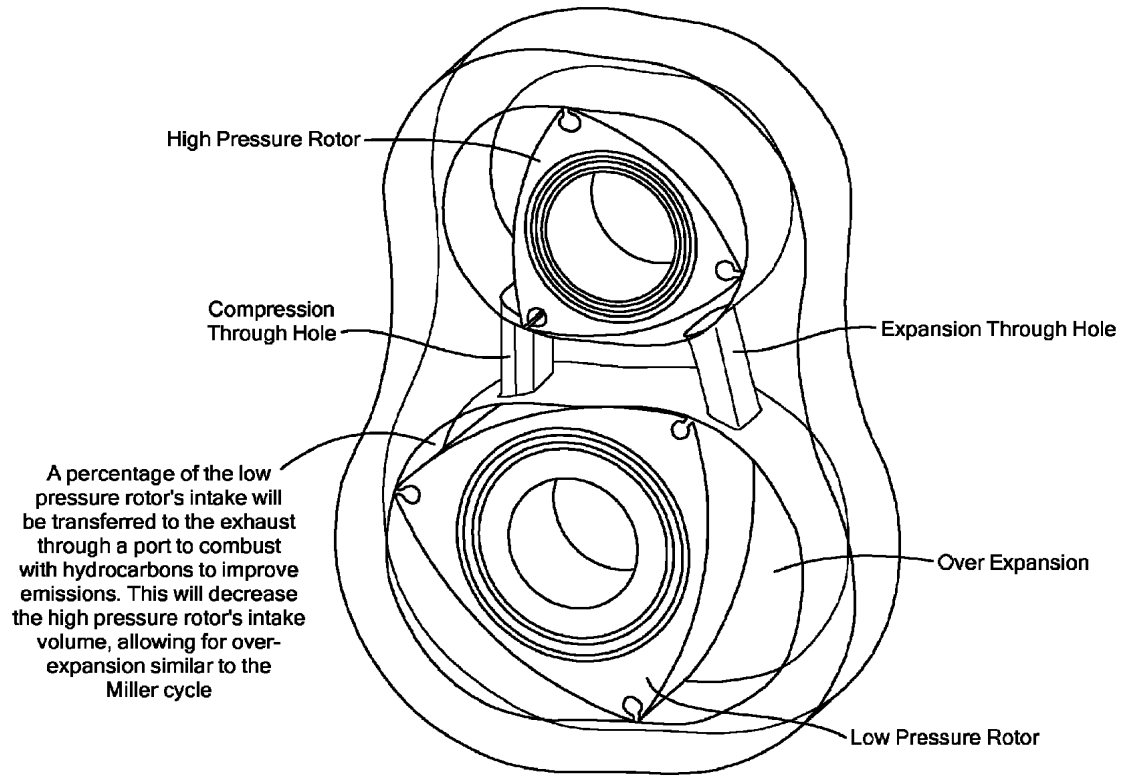
Two Pistons - Two-Stage Embodiment.
