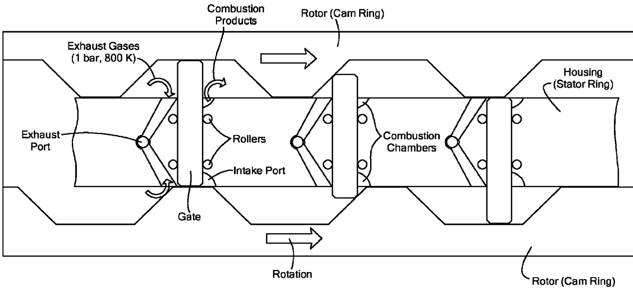
Two Rotors/Multiple Gates Embodiments
