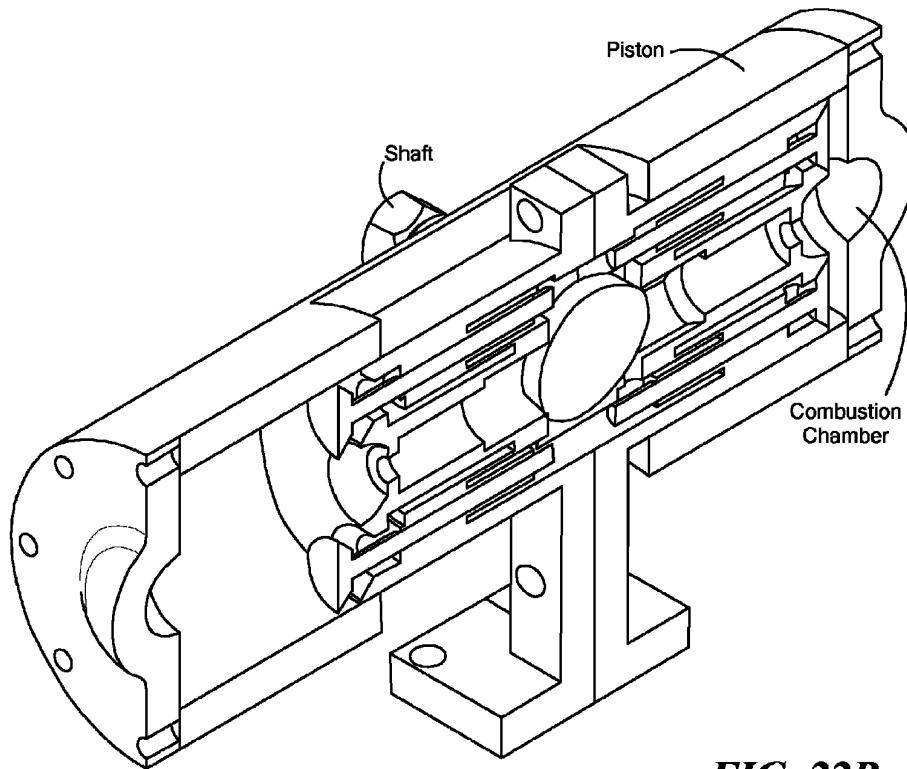
Single Piston (2-Cylinder) Embodiments
