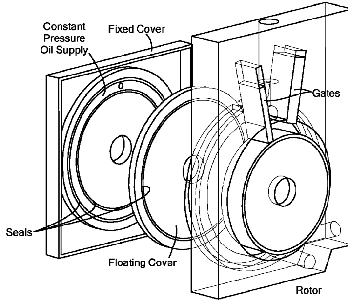
Exploded Back View, showing seals
