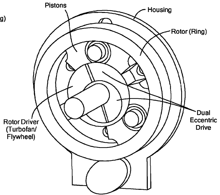
Dual Eccentric Drive
