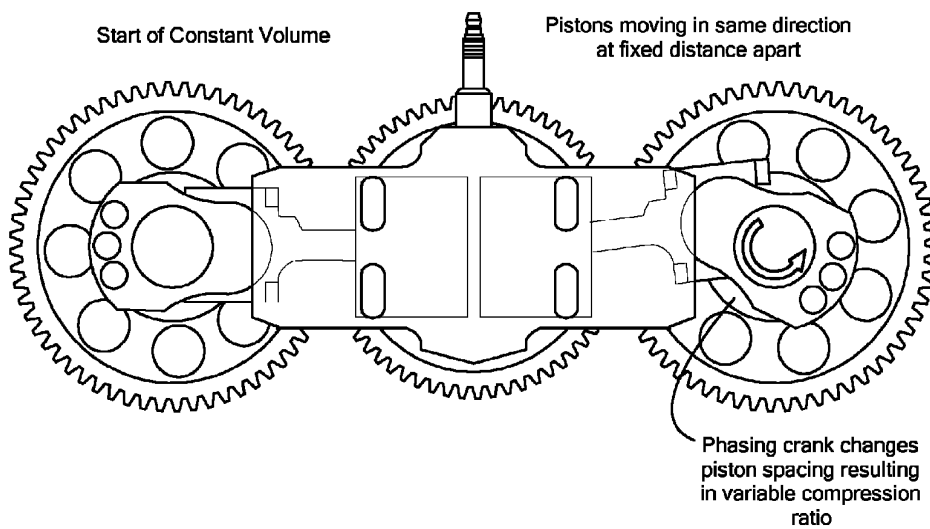
Two Pistons - Opposed Pistons Embodiment. Compression Stroke
